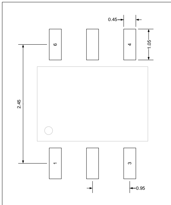
Figure 10-4 SOT23-6 recommend footprint
